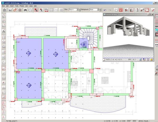
Superstructure Input
