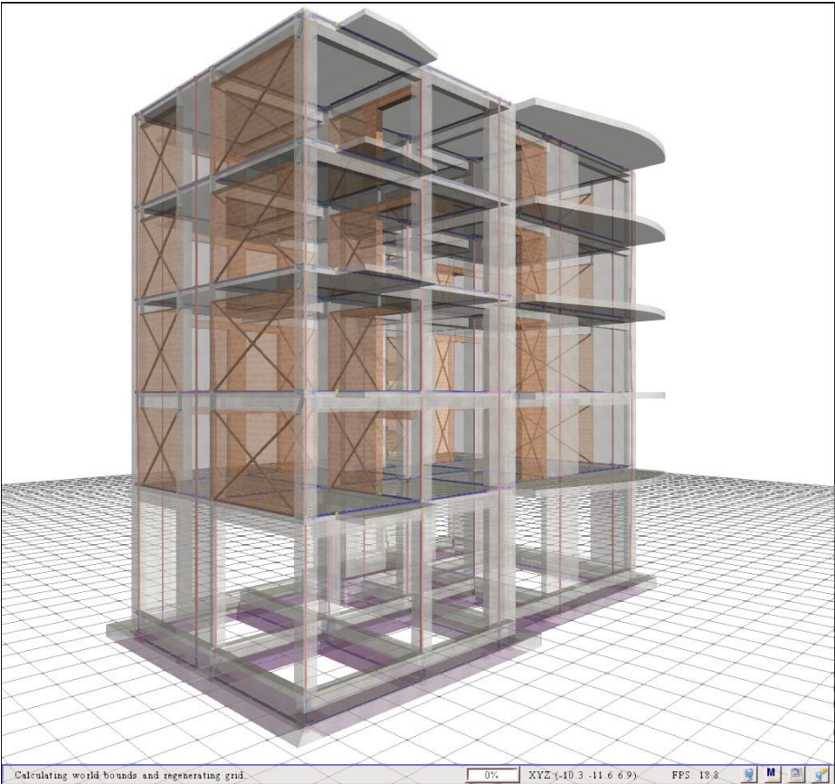
(21) Optional modelling of masonry with a couple of diagonal bar elements. In each loading condition, only the bar element under compression is taken into account
